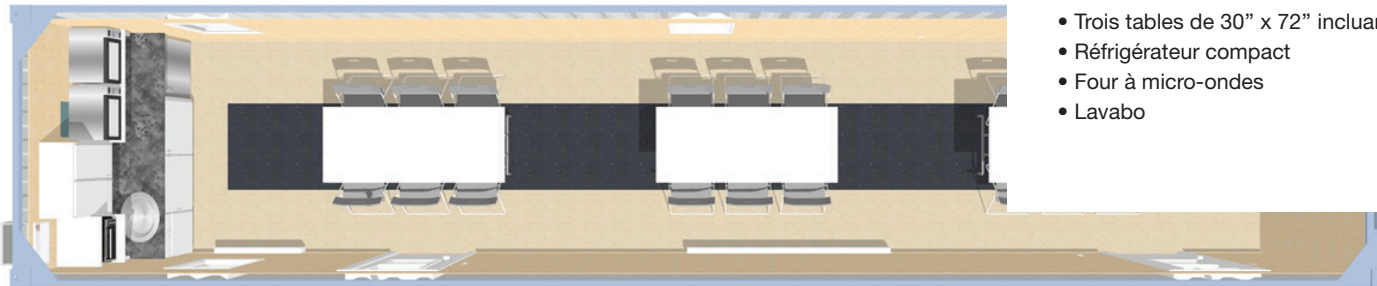
PLAN
